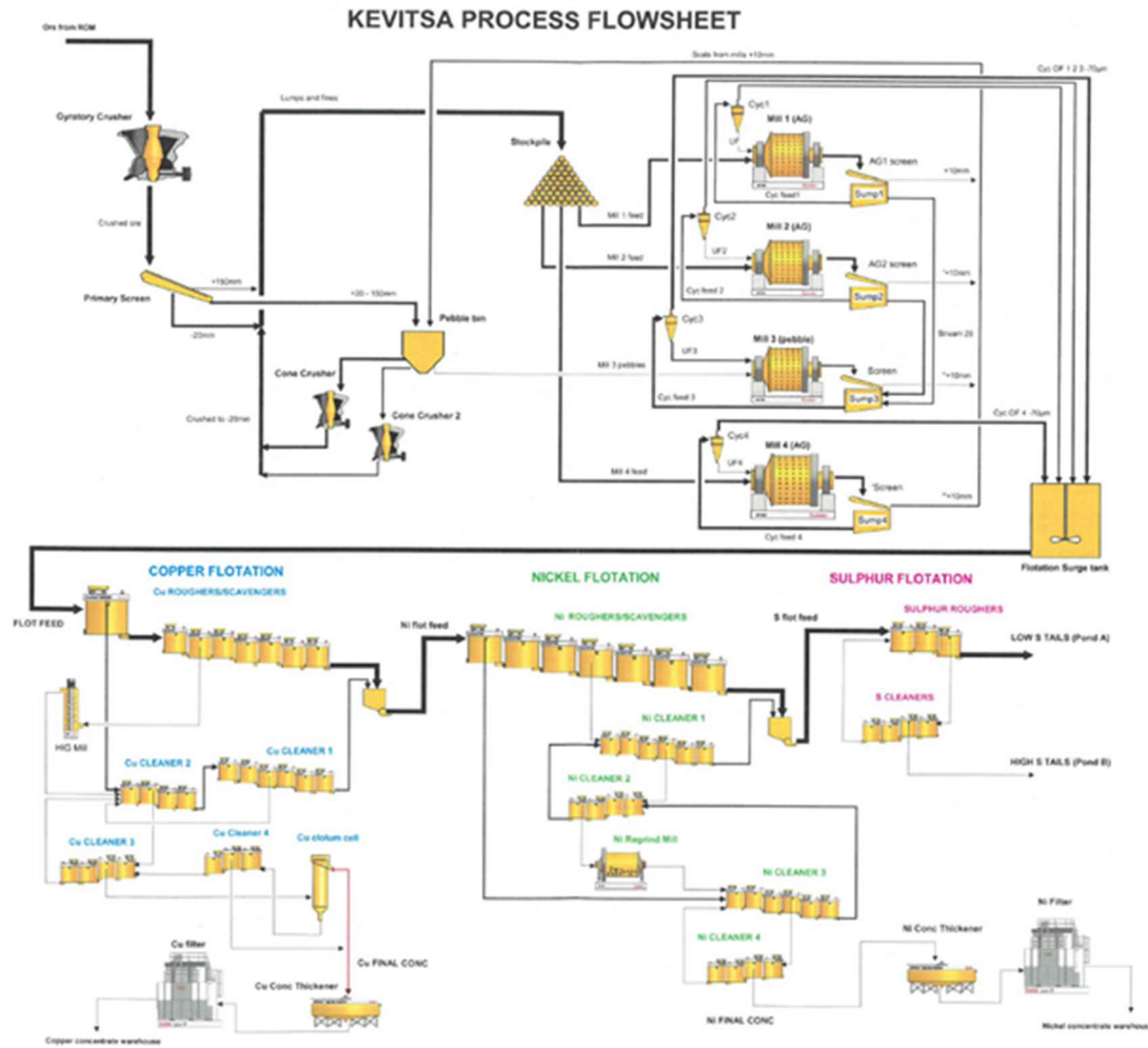
Figure 7. Simplified flowchart of the Kevitsa Mine process
