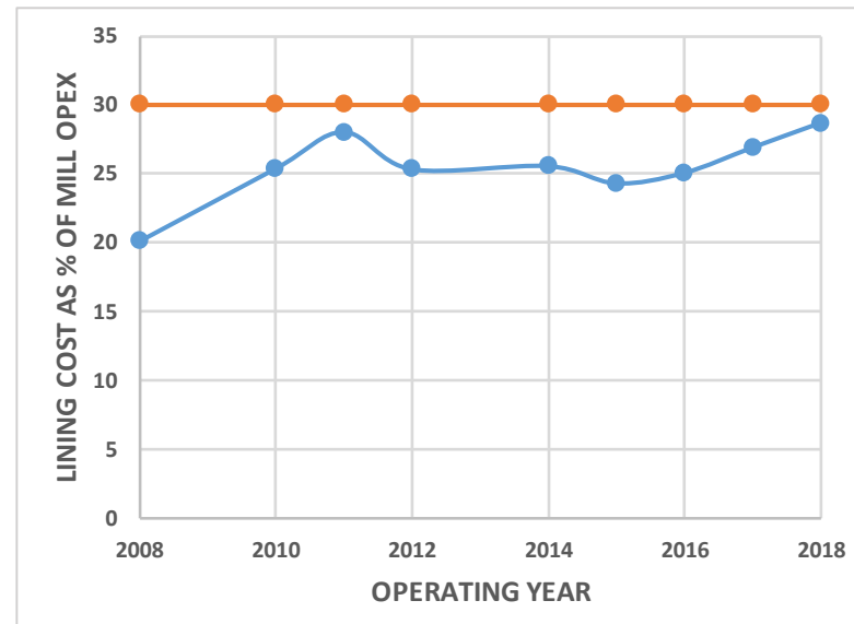
ACTUAL LINER COST SHARE IN AG MILL OPEX AGAINST A VARIABLE INDUSTRIAL ELECTRICITY TARIFF
