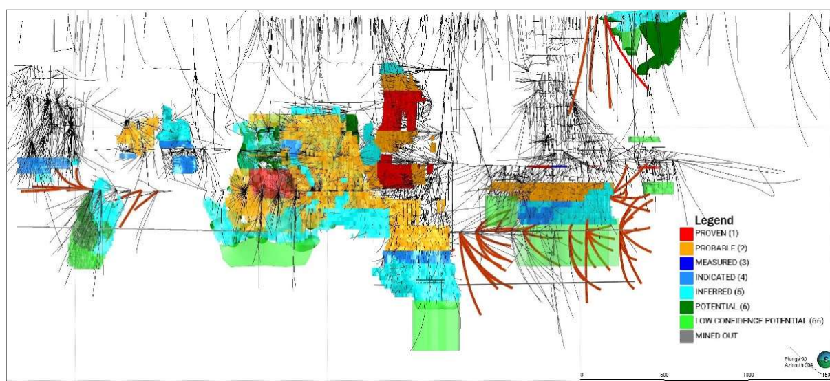
Figure 3-7. Front view with 2023 Reserves & Resources, that was used as a base for 2024 Near mine drilling program (in red).
