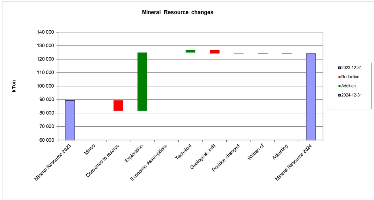
Figure 3-12. Changes to Mineral Resources between 2023-12-31 (leftmost column) and 2024-12-31 (rightmost column). The other columns show the causes for reduction (in red) and addition (in green) of tonnage. Note that the scale of the y-axis has been adjusted and starts at 60 000 kton.
