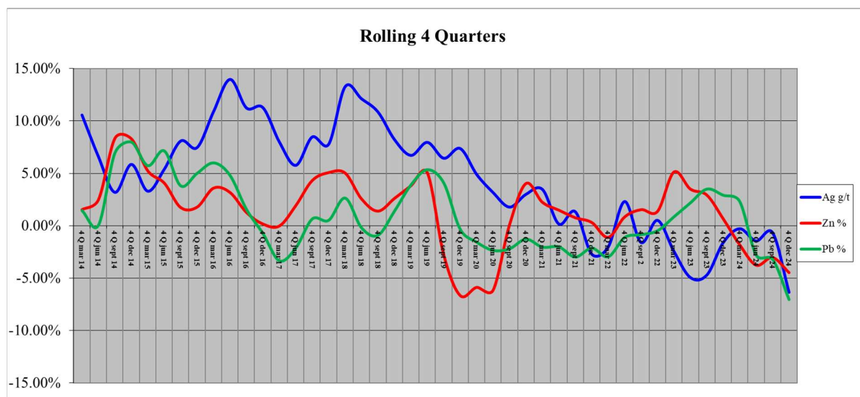
Figure 3-16. Metal grades in processed ore vs metal grades of the mined ore based on the block model, over a ten-year period.
