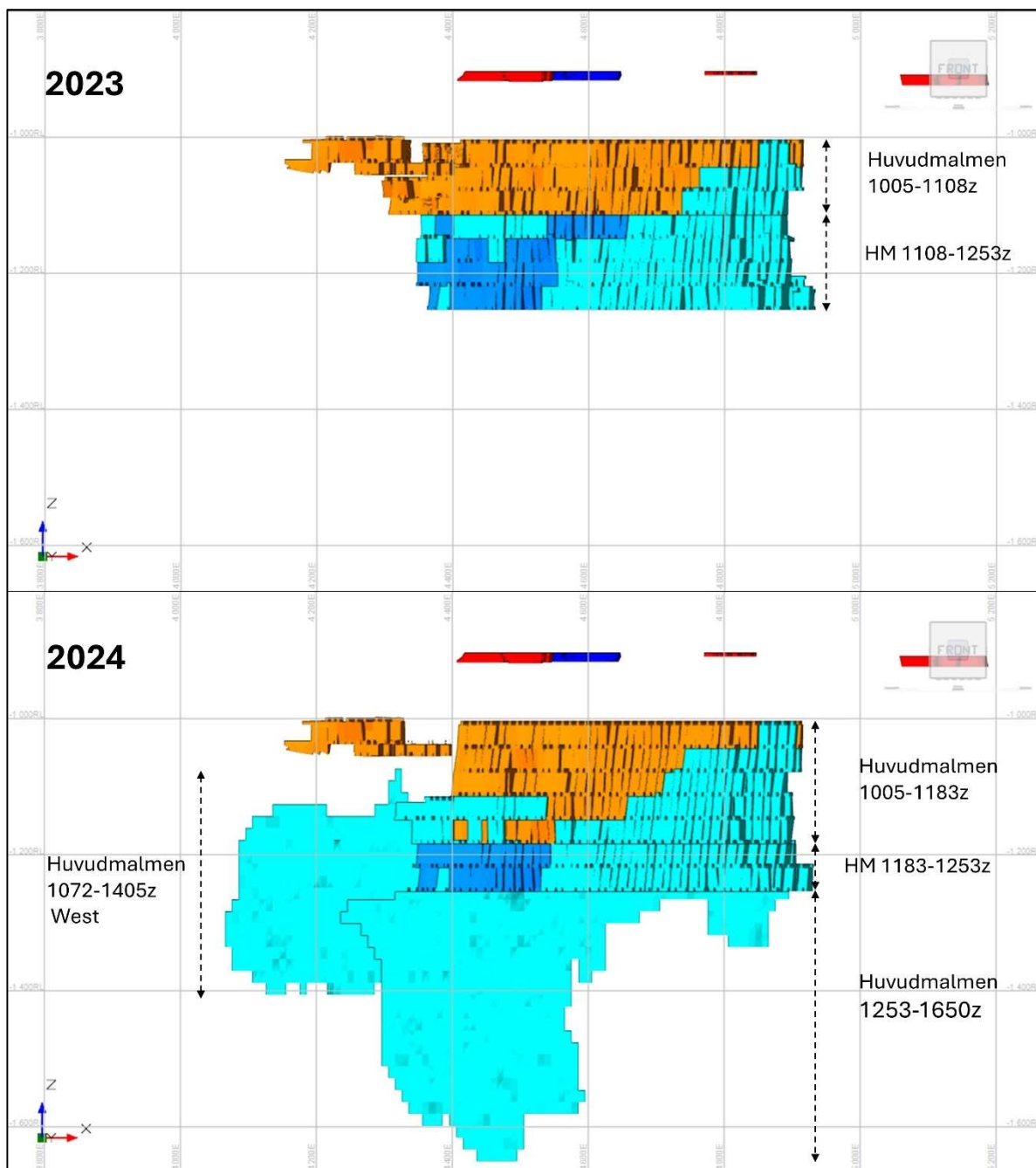
Figure 3-13. Changes in resources and reserves in Huvudmalmen. The image is a front view of the Huvudmalmen and Kaspersbo ore body, looking North.
